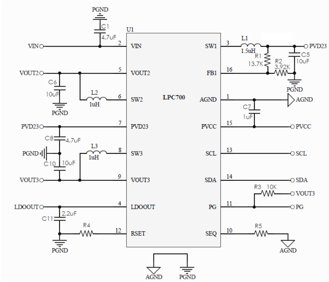
Figure 1. Typical Application
