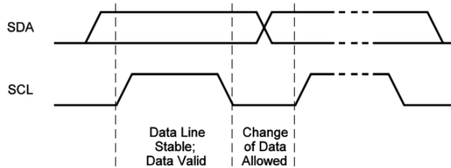
Figure4: Bit Transfer on the I2C
