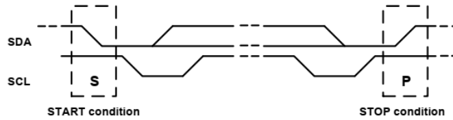
Figure 5: START & STOP Conditions
