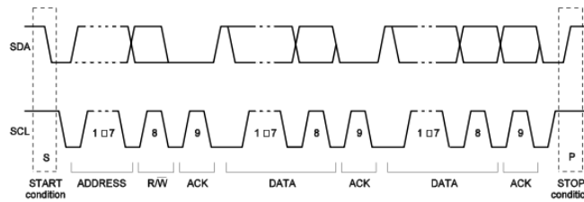
Figure 6: A Complete Data Transfer
