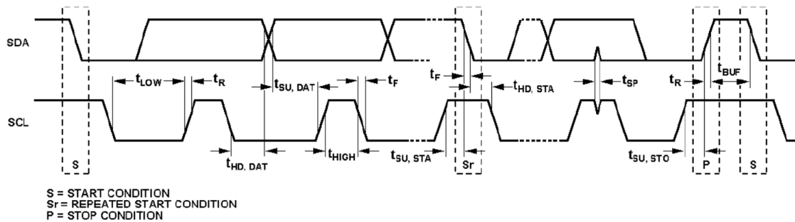
Figure2: I2C Compatible Interface Timing Diagram
